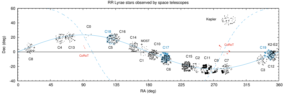
Fig. 1: RR Lyrae stars observed by various space missions. Black and blue points show targeted and proposed Kepler and K2 observations, red points are CoRoT targets, and cross marks the single MOST target.
