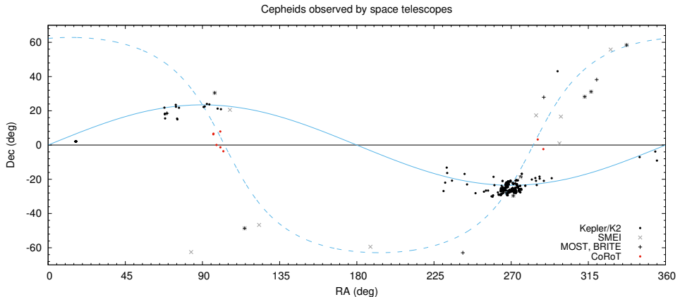
Fig. 2: Cepheid stars observed by various space missions. Notation is similar to Fig. 1. The only target missing from this map is Polaris.
